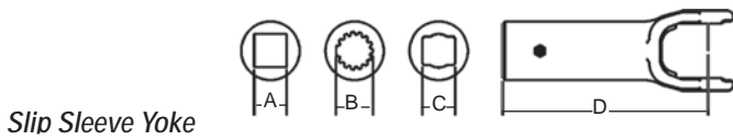
1" x 1 1/8" Tube
