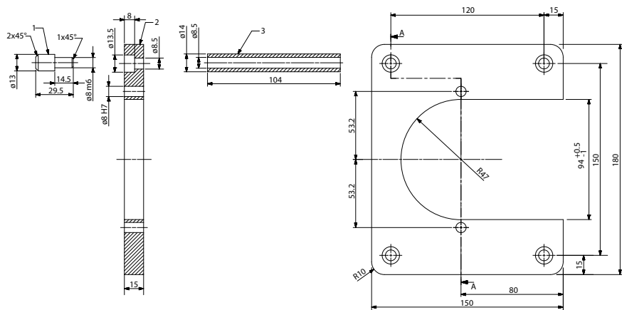
Figure 3: A2 flange
