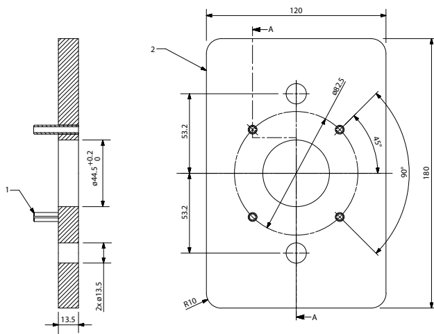
Figure 4: C-flange
